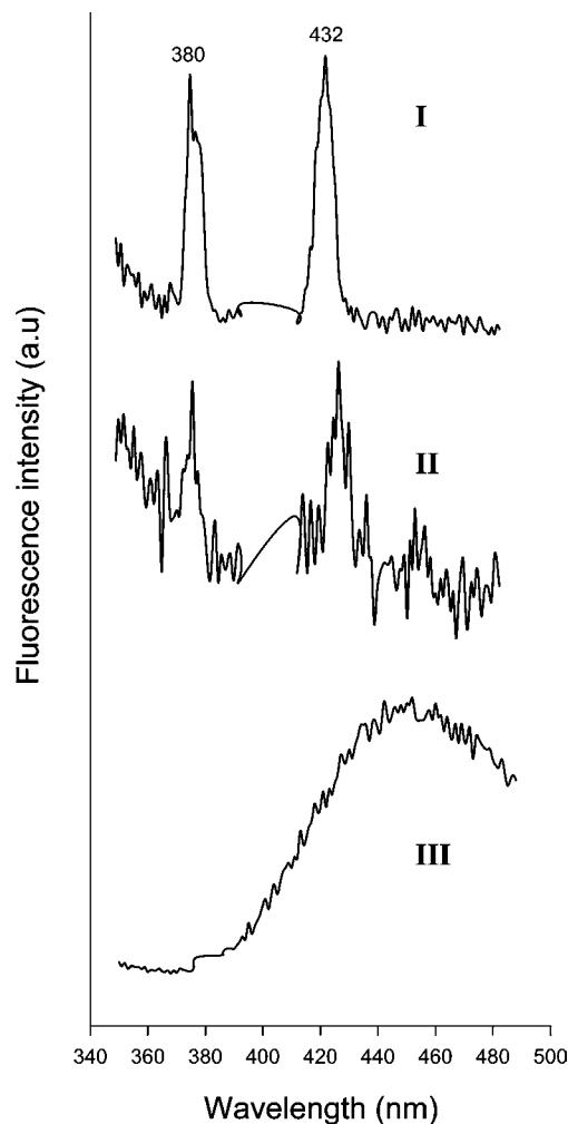
Figure 3. Fluorescence spectra of NAD standard solution (I, 10 ppm), NAD in the extract of live larvae reared on diet A (II), and dead larvae reared on diet D (III). Excitation wavelength was at 380 nm and emission at 432 nm.
