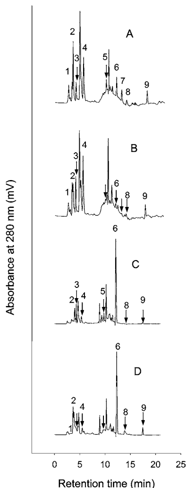
Figure 1. HPLC chromatograms (method 1) of metabolites in the extracts of live larvae A ( Figure 1A ) and the corresponding spent diet A ( Figure 1C ), and dead larvae D ( Figure 1B ) and the corresponding spent diet D ( Figure 1D ) (second instar, 7-day-old larvae). Diet A contained 20 \mu\text{g/g} of nicotinic acid and 707 \mu\text{g/g} of nine other vitamins. Diet D contained no nicotinic acid but 707 \mu\text{g/g} of the nine other vitamins. 1, citric acid; 2, p -aminobenzoic acid; 3, nicotinic acid; 4, pyridoxine; 5, nicotinamide; 6, folic acid; 7, riboflavin; 8, pantothenic acid; and 9, inositol.
