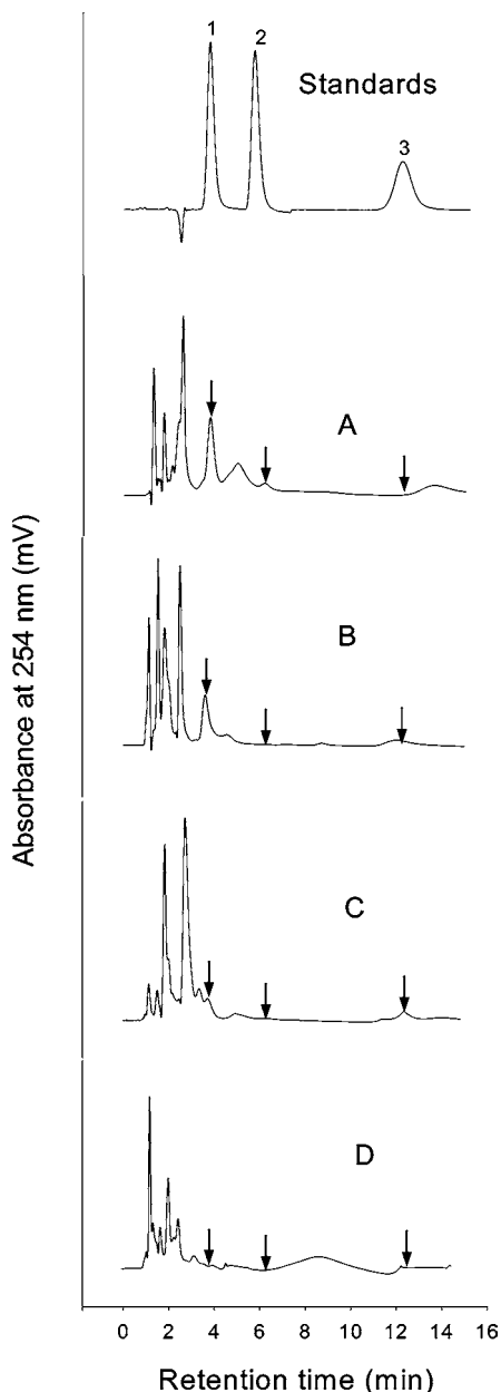
Figure 2. HPLC chromatograms (method 2) of nicotinic acid, nicotinamide, and NAD in the extracts of live (A, B, and C) and dead larvae (D). Standards: a mixture of standard nicotinamide (1), nicotinic acid (2), and NAD (3) at each 10 \mu\text{g/mL} , injection volume of 20 \mu\text{L} . Larvae were reared on diets A (A, 20 \mu\text{g/g} of nicotinic acid + 707 \mu\text{g/g} the nine other vitamins), B (B, 2 \mu\text{g/g} of nicotinic acid + 707 \mu\text{g/g} of the nine other vitamins), C (C, no nicotinic acid nor the nine other vitamins), and D (D, no nicotinic acid but 707 \mu\text{g/g} of the nine other vitamins) as described in Table 2.
